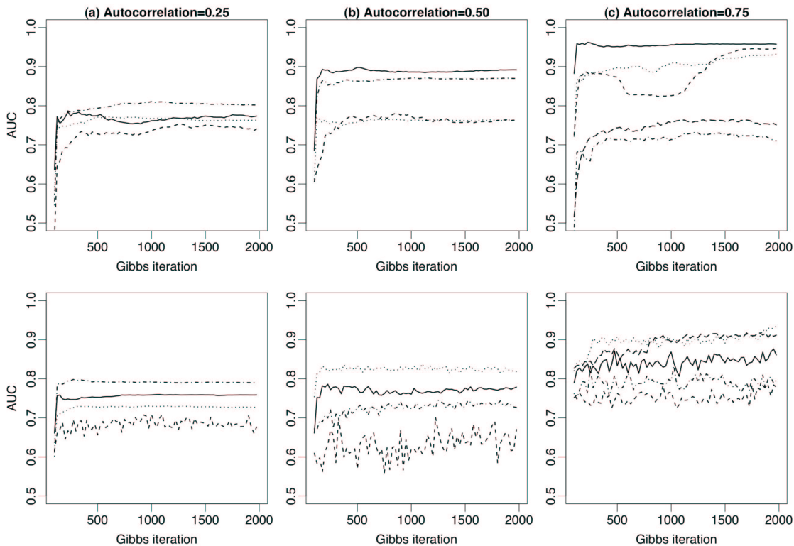
Figure 8: Gibbs convergence rates for five different trials of RDN_{RPT} (top row) and RDN_{RBC} (bottom row).
