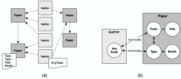
Figure 2: Example (a) data graph and (b) model graph.
