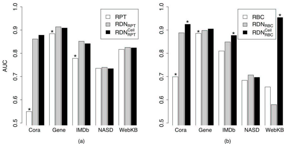
Figure 15: AUC results for (a) RDN_{RPT} and RPT, and (b) RDN_{RBC} and RBC. Asterisks denote model performance that is significantly different ( p < 0.10 ) from RDN_{RPT} and RDN_{RBC} .
