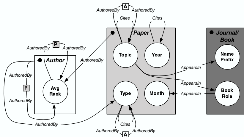
Figure 10: RDN for the Cora data set.
