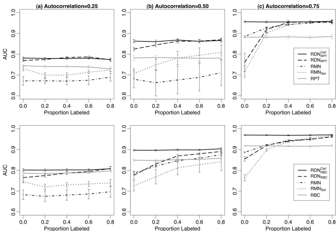
Figure 7: Evaluation of RDN inference.
