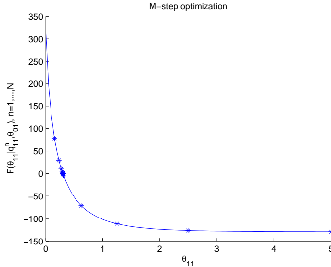
Figure 2: A summary of iterative optimization steps for the variational learning method.
