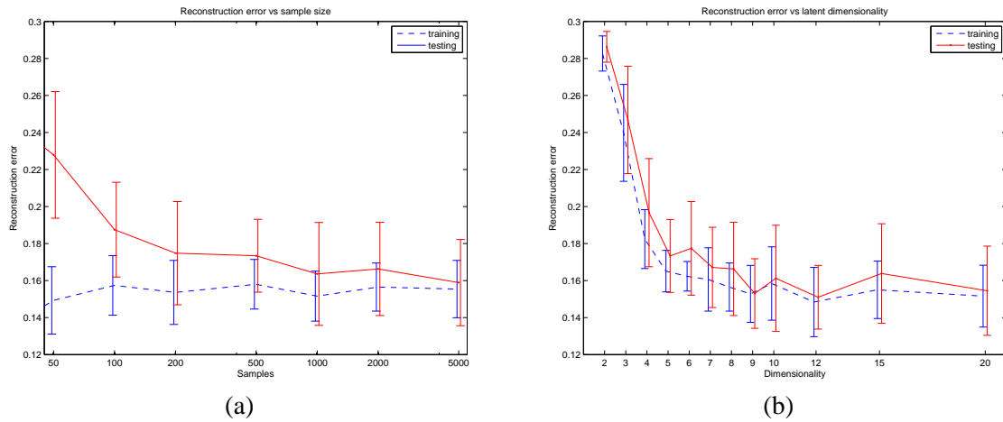
Figure 9: (a) Average data reconstruction errors obtained for varied training sample sizes. (b) Average data reconstruction error plotted against the number of assumed latent sources. All values are averaged over 50 runs.
