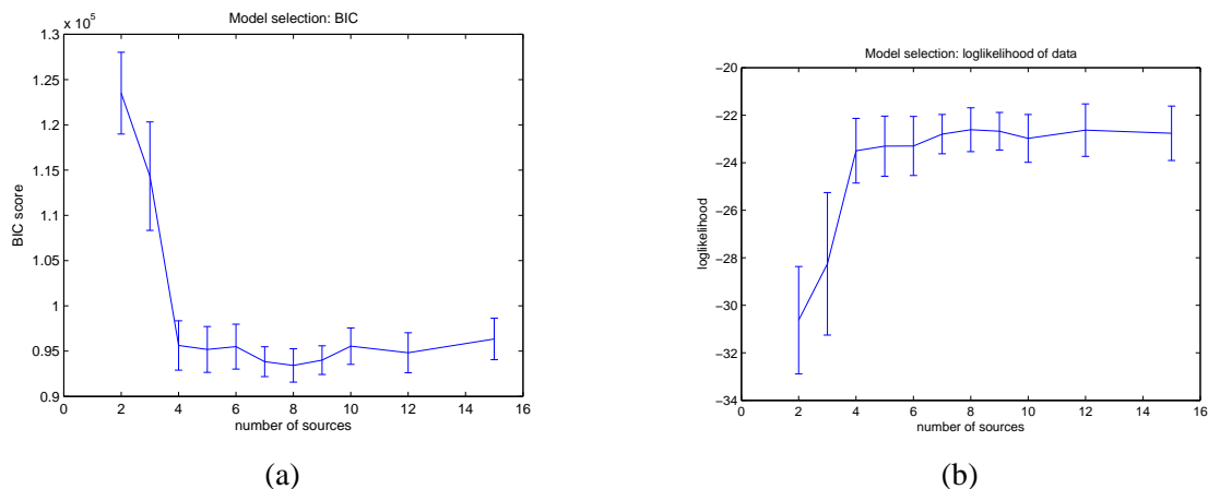
Figure 7: (a) The average BIC scores for the models with varied number of sources. (b) The average log-likelihood of data for model with varied number of sources. In both cases, the true number of sources K is fixed at 8. Averages are calculated from 20 trials (one-standard-deviation bars are shown). In each trial, the model was learned using 2000 data points. The BIC reaches its optimal value at, and log-likelihood levels at 8 sources, which corresponds to true number of sources.
