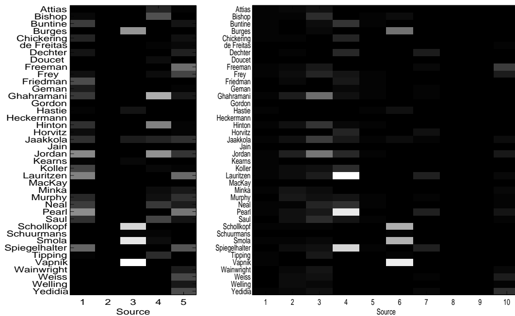
Figure 12: A result of noisy-or component analysis on the citation data set. The columns visualize the parameters of the noisy-or loading matrix after they are rescaled by the prior of the source. Black fields correspond to 0s in the loading matrix, while white ones correspond to 1s.
