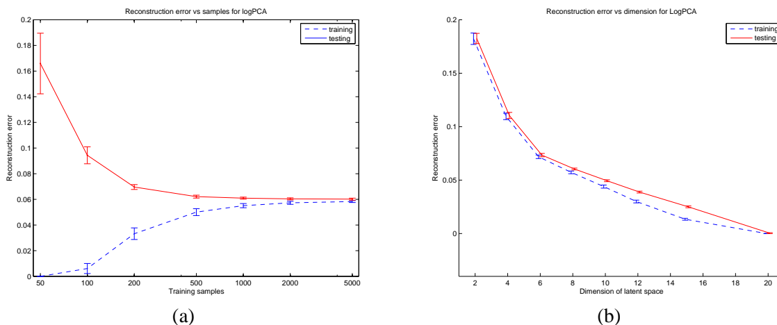
Figure 10: Reconstruction errors achieved by the logistic PCA, a) as they vary with training set size (fixed size testset), and b) as they vary with the latent dimension of the model.
