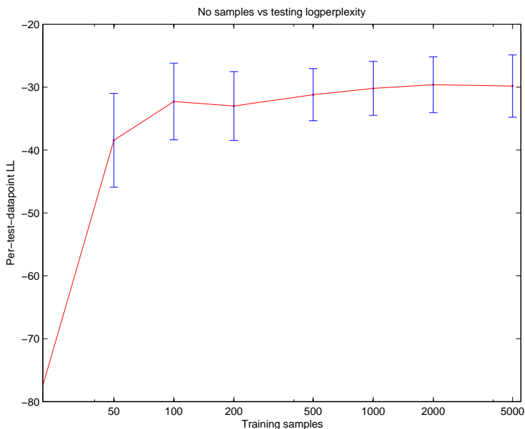
Figure 6: Average log-likelihoods of NOCA models on testing sets. The models are learned from training sets of size 50, 100, 200, 500, 1000, 2000 and 5000. The averages are over 50 trials. One-standard-deviation error bars are shown. The increase in the log-likelihood illustrates the improvement in the model recovery with an increasing sample size.
