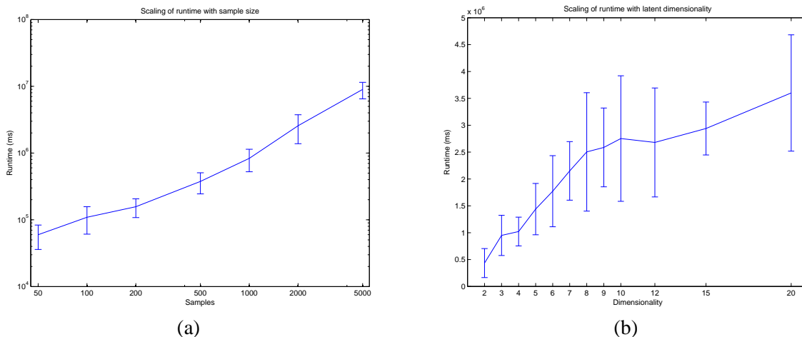
Figure 8: (a) Runtimes of NOCA as they scale with increasing size of the training set. K is fixed at 8. (b) Scale-up with the number of assumed latent sources, the data set size is fixed at 2000.
