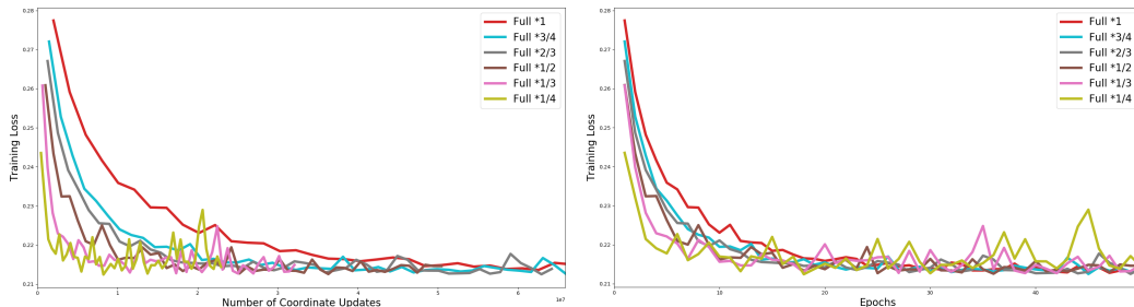
Figure 1: ijcnn1 data set for different fraction of non-zero set
