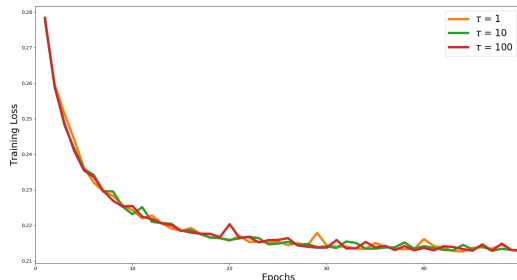
Figure 2: ijcnn1 data set for different \tau with the whole non-zero set
