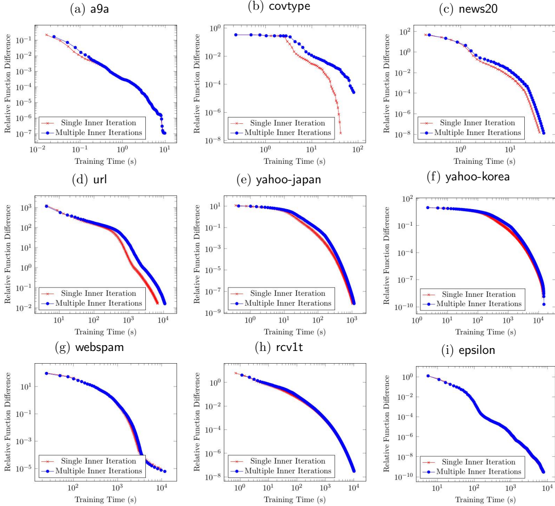
Figure 3: Comparison between single inner iteration and multiple inner iterations variants of the common-directions method. We present training time (in log scale) of logistic regression with C = 10^3 .
