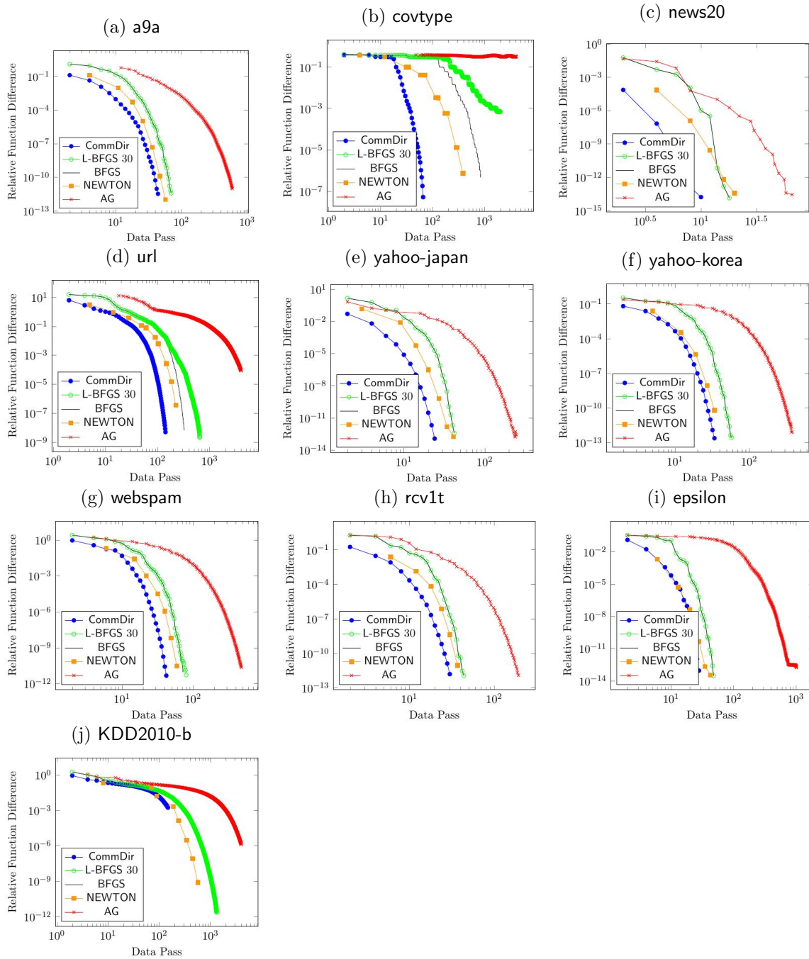
Figure 16: Number of data passes of L2-loss SVM with C = 10^{-3} .
