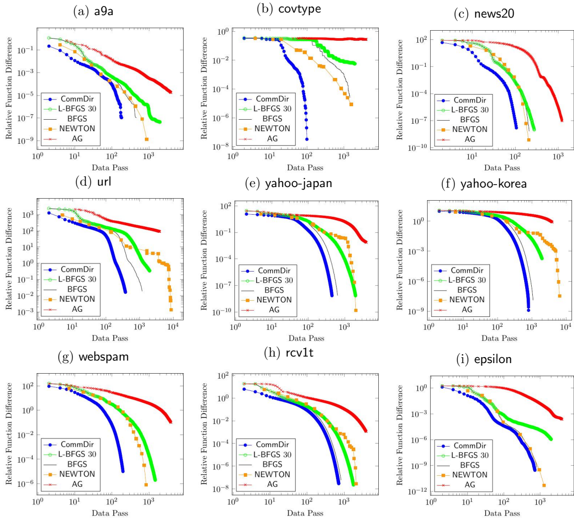
Figure 12: Number of data passes of logistic regression with C = 10^3 .
