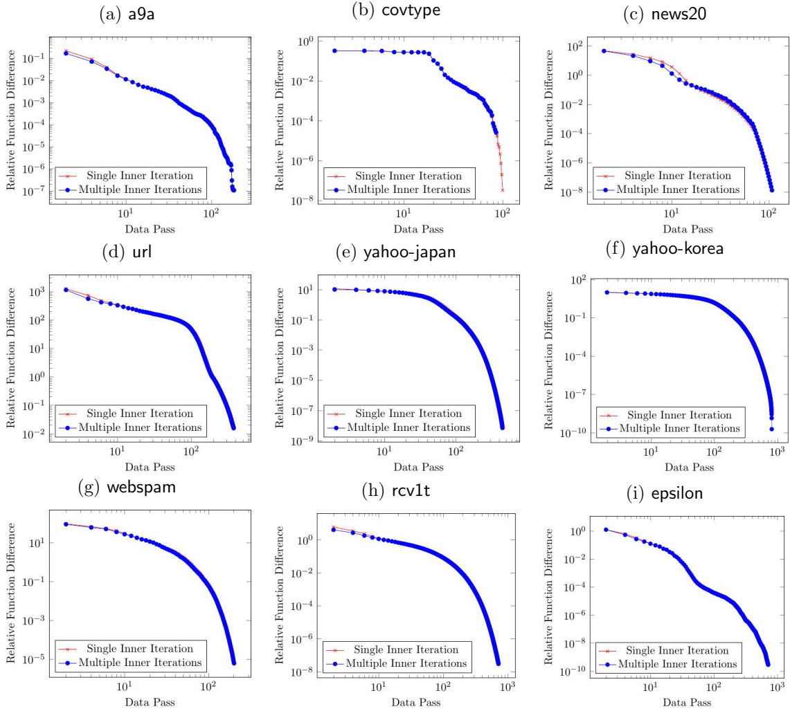
Figure 6: Comparison between single inner iteration and multiple inner iterations variants of the common-directions method. We present data passes (in log scale) of logistic regression with C = 10^3 .
