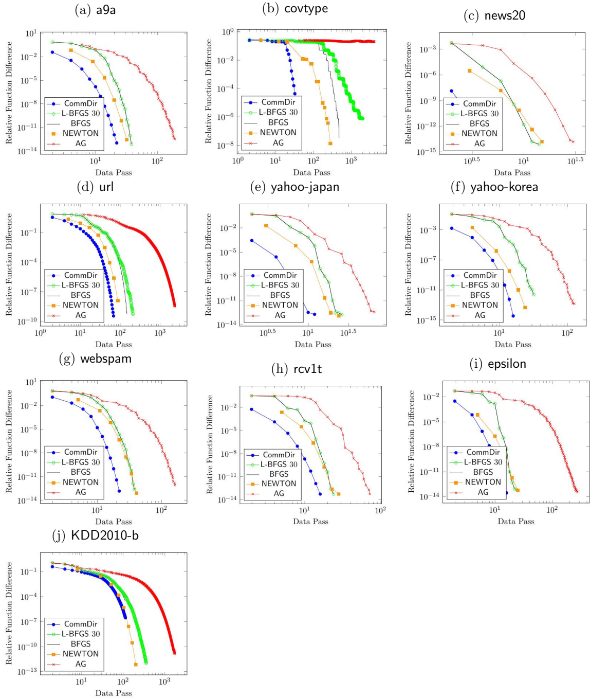
Figure 10: Number of data passes of logistic regression with C = 10^{-3} .
