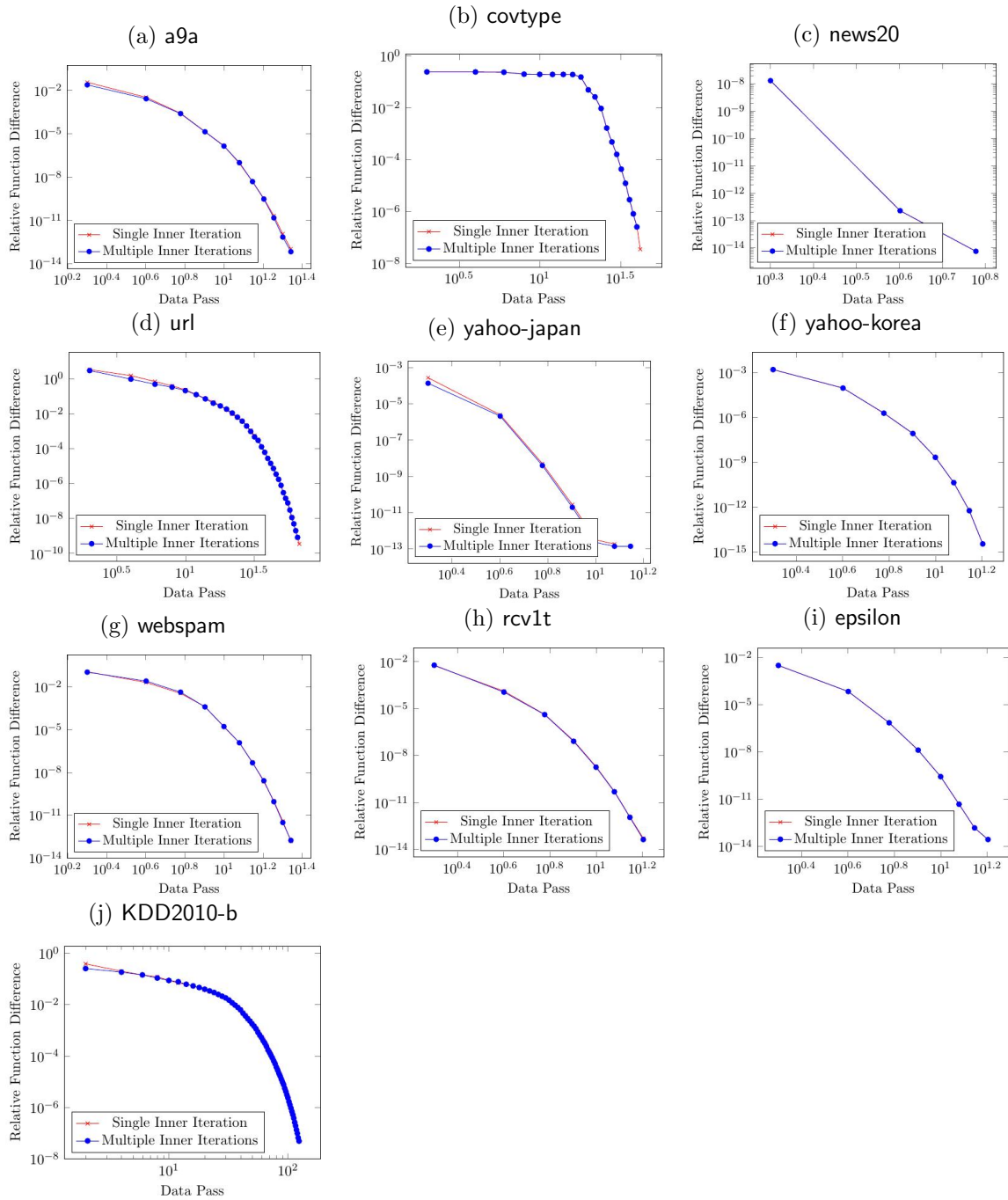
Figure 4: Comparison between single inner iteration and multiple inner iterations variants of the common-directions method. We present data passes (in log scale) of logistic regression with C = 10^{-3} .
