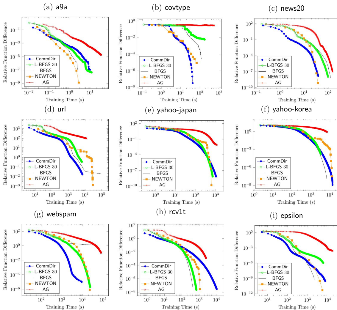
Figure 9: Training time of logistic regression with C = 10^3 .
