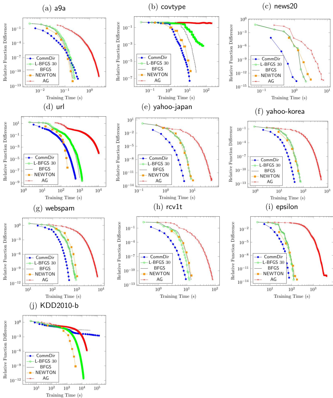
Figure 13: Training time of L2-loss SVM with C = 10^{-3} .
