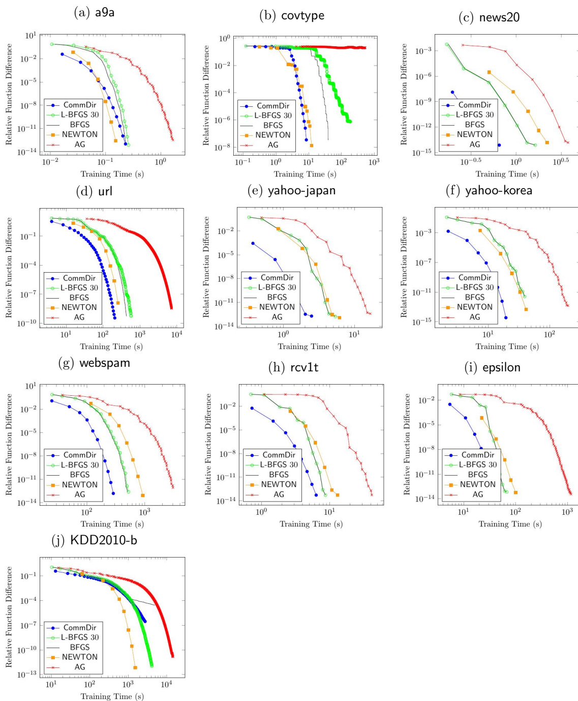
Figure 7: Training time of logistic regression with C = 10^{-3} .
