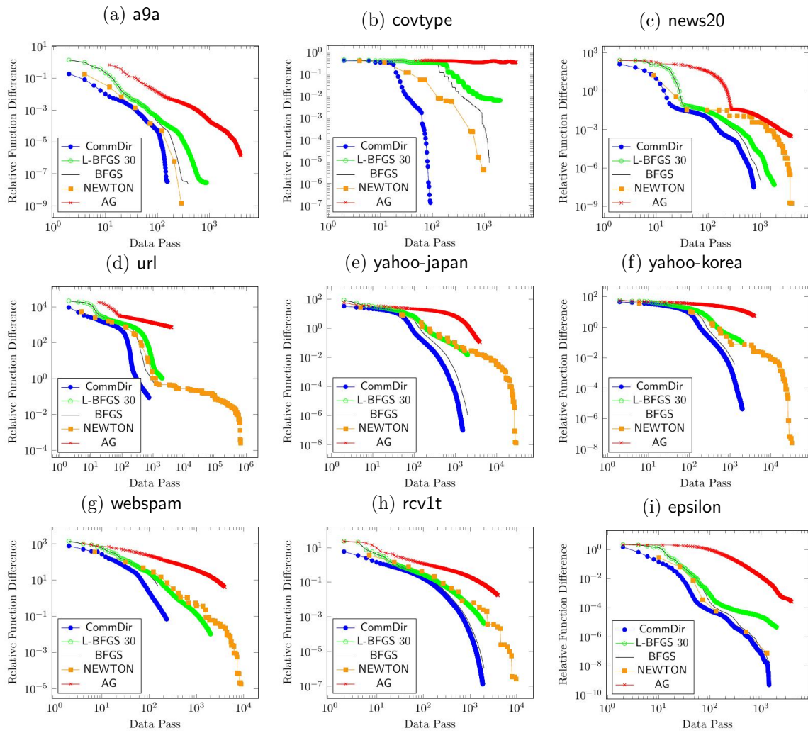
Figure 18: Number of data passes of L2-loss SVM with C = 10^3 .
