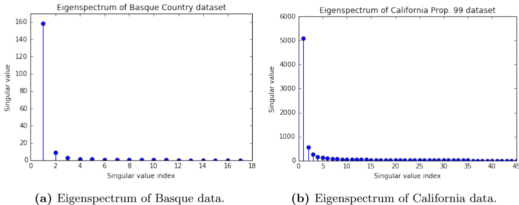
Figure 1: Eigenspectrum
