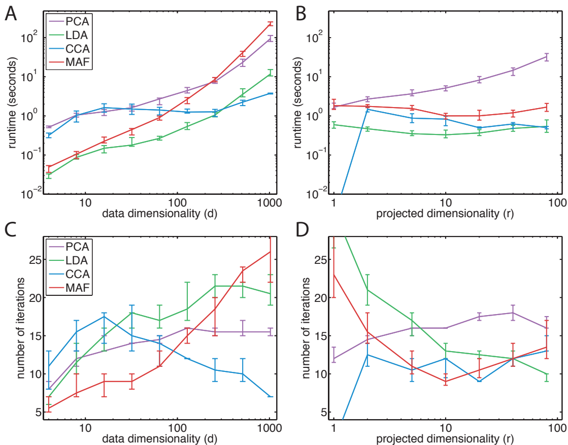
Figure 3: Computational cost of direct optimization of linear dimensionality reduction objectives. Data sets are the same as those in Figure 2. The vertical axis in panels A and B denotes runtime in seconds. Panels C and D show the same data by the number of solver iterations.
